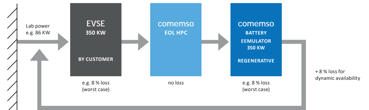
Example of conducting a 350 kW charging test with a lower grid connection, using the battery emulator's regenerative power capability.
