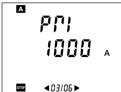
Figure 49: Display of parameter relating to the effective primary current of the intensity transformer.
