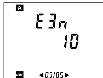
Figure 51: Display of the parameter concerning the sensitivity used on the clamp.
